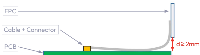
Vertical mounted
