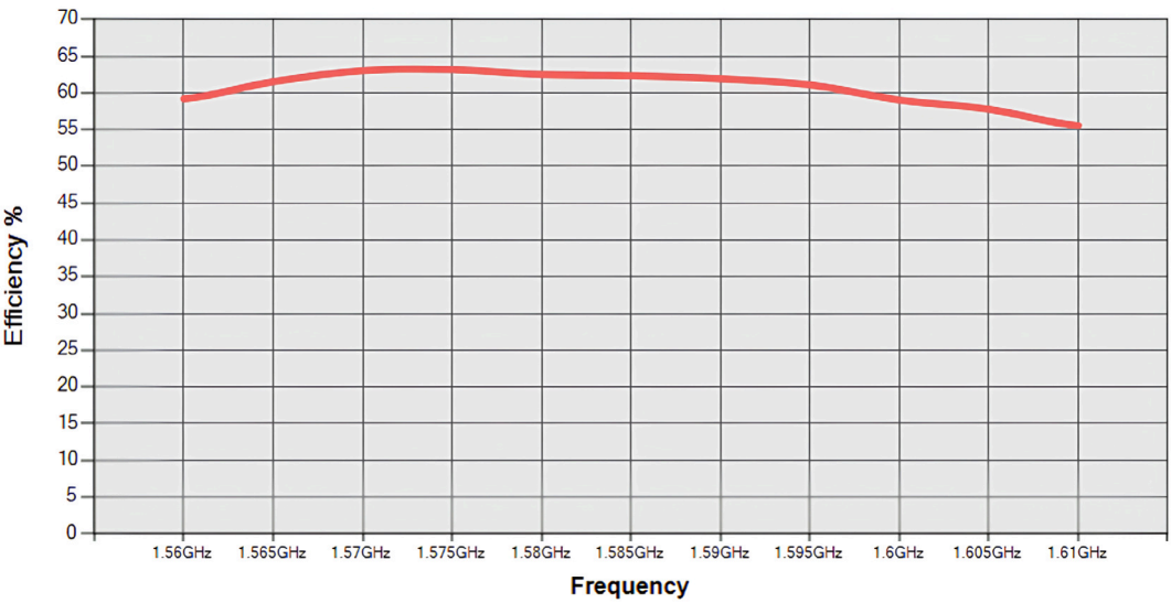
All data measured on Antenova's evaluation PCB Part No. SR4G013-EVB-1.
