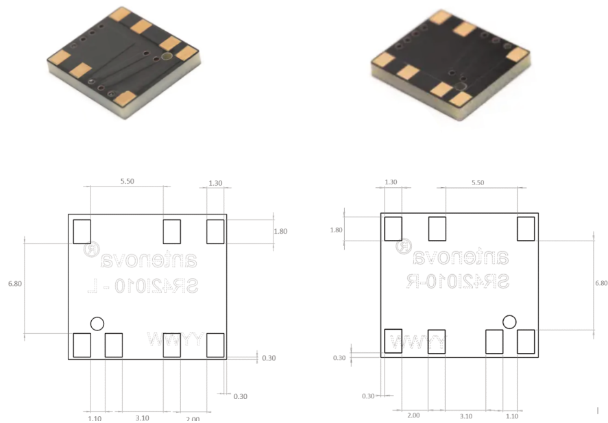
Bottom view
