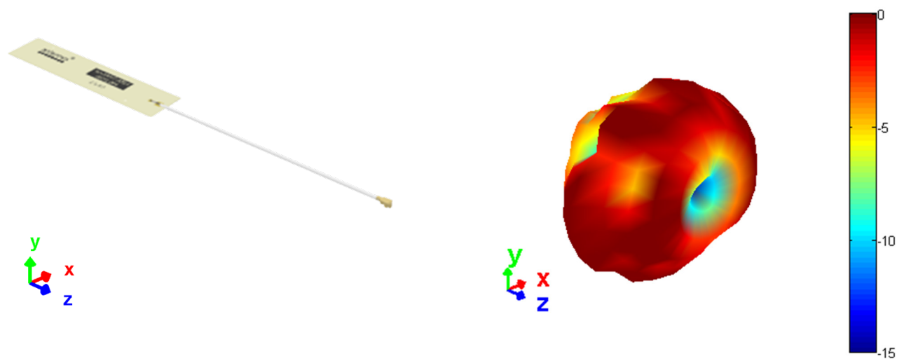
3D pattern at 2340 MHz
