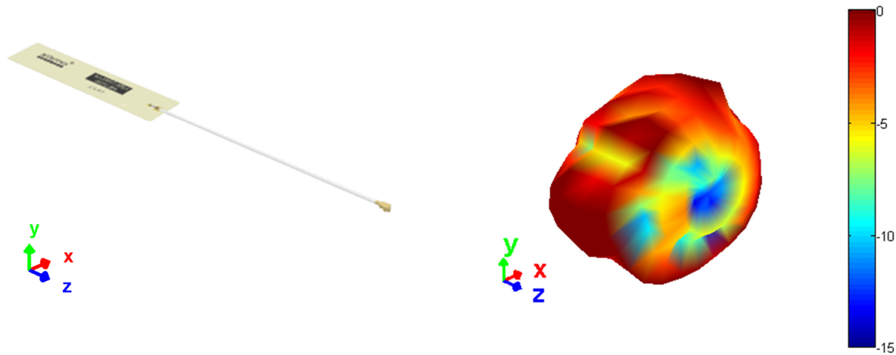
3D pattern at 2600 MHz
