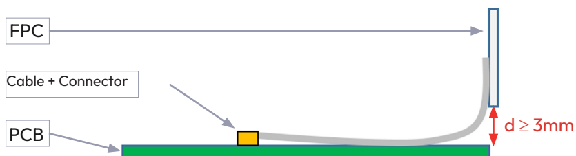
Vertical mounted
